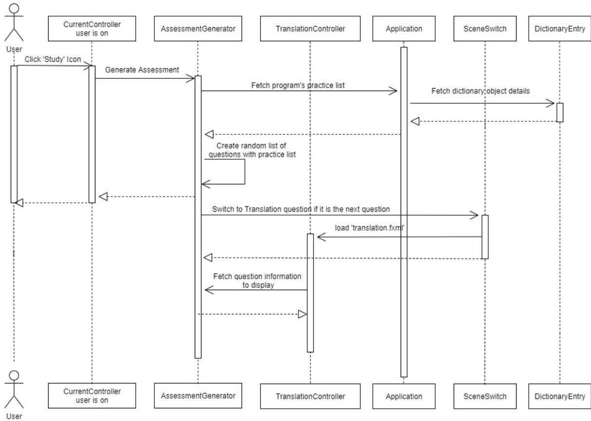
Figure 9: Sequence diagram for the 'Translation' test
