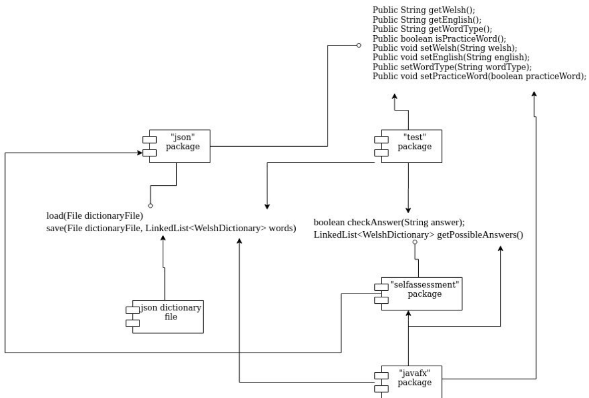
Figure 1: Component diagram of the Welsh Vocabulary App
