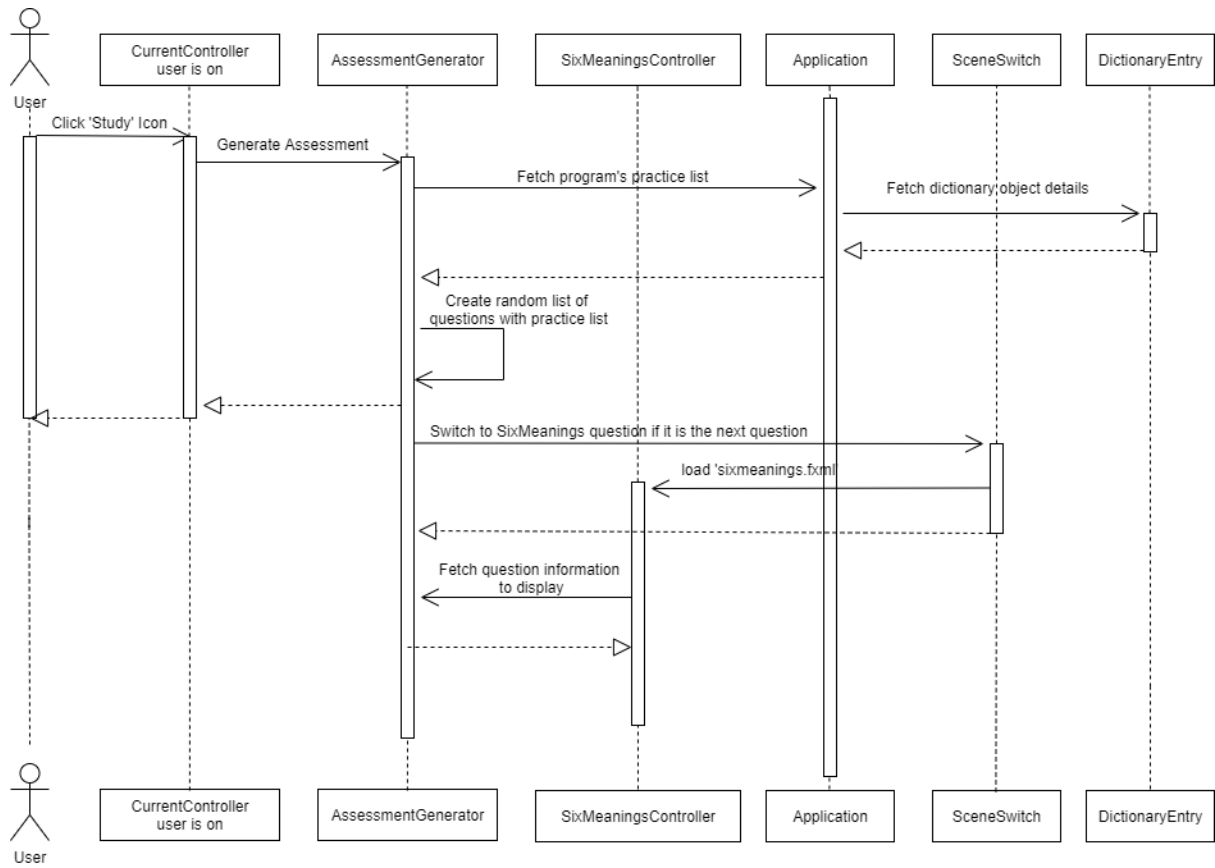
Figure 8: Sequence diagram for the '6 Meanings' test
